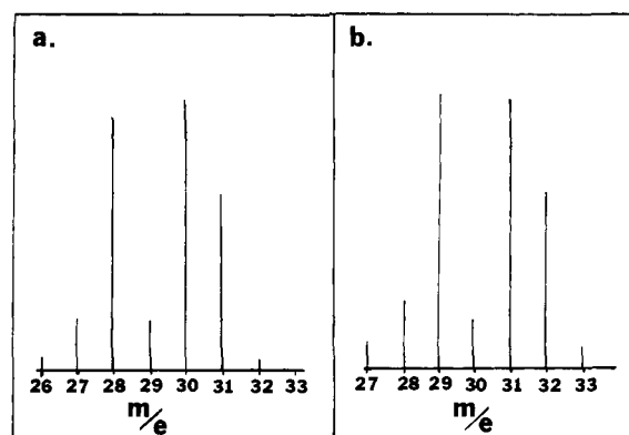
Figure 3. Mass spectra obtained for (a) methylamine standard in \text{NH}_3 and (b) Nitrogen-15 labeled methylamine from photoreaction. (See Experimental Section for details.)
