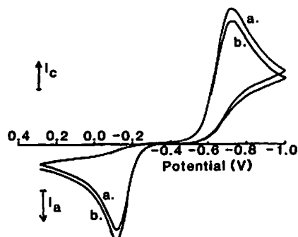
Figure 7. Simulated cyclic voltammogram of 2 based on an ECE/EE 1 (DISP) mechanism. E_1 = -0.18 V, E_2 = 0.0 V, E_3 = -2.5 V, \psi_1 = 0.002 , \psi_2 = 0.1 , \psi_3 = 100 , \alpha_1 = 0.52 , \alpha_2 = 0.30 , \alpha_3 = 0.5 . First (a) and second (b) scans are shown.
