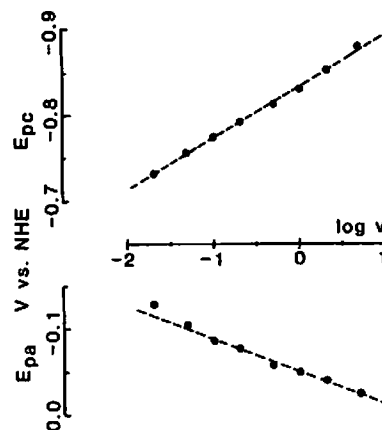
Figure 3. Plots of peak potential for the reduction of 0.94 mM 2 and the oxidation of the dianion of 2 vs. \log v in THF/0.4 M (TBA)BF 4 . For cathodic scan, slope = 56 mV; for anodic scan, slope = 39 mV.
