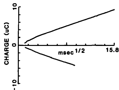
Figure 6. Chronocoulometric Q vs. t^{1/2} plot of a 1.61 mM solution of 5 in freshly distilled THF/1 M (TBA)BF 4 . The electrode was pulsed from -0.2 to -2.1 V and back. Forward scan: slope = 0.547 \mu\text{C}/\text{ms}^{1/2} ; intercept = 0.734 \mu\text{C} . Reverse scan: slope = 0.524 \mu\text{C}/\text{ms}^{1/2} ; intercept = 0.388 \mu\text{C} .
