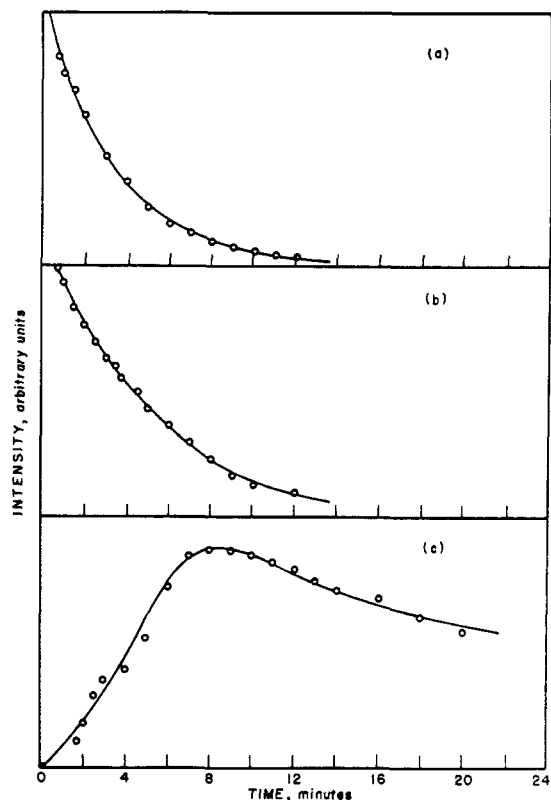
Figure 4. Time dependence of spectral components in 10 mM anthracene solutions: (a) ECL emission at 412 m \mu ; (b) ECL emission at 470 m \mu ; (c) fluorescence emission at 470 m \mu , excited by 420-m \mu radiation.
