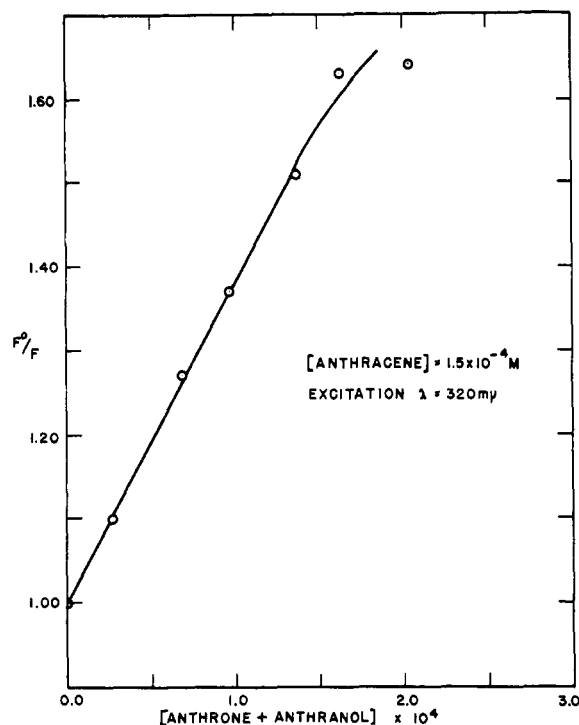
Figure 7. Sensitization of anthranol fluorescence at 457 m\mu by anthracene.
