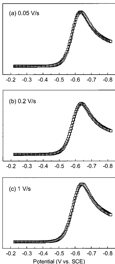
Figure 4. Scan rate variations of cyclic voltammograms by the experimental (—) and digital simulations (□) of 0.15 mM QDI in \text{CHCl}_3/\text{CH}_3\text{CN} (4:1, v/v), (electrolyte: 0.1 M TBAPF 6 ): (a) = 0.05, (b) = 0.2, and (c) = 1 V/s at a 3.4 mm diameter Pt electrode. The experimental data were corrected for Ohmic drop. Simulation parameters: reduction reaction E_{1r} = -0.58 V vs SCE, E_{2r} = -0.62 V vs SCE, \alpha = 0.5 , k_s = 0.5 cm/s.
