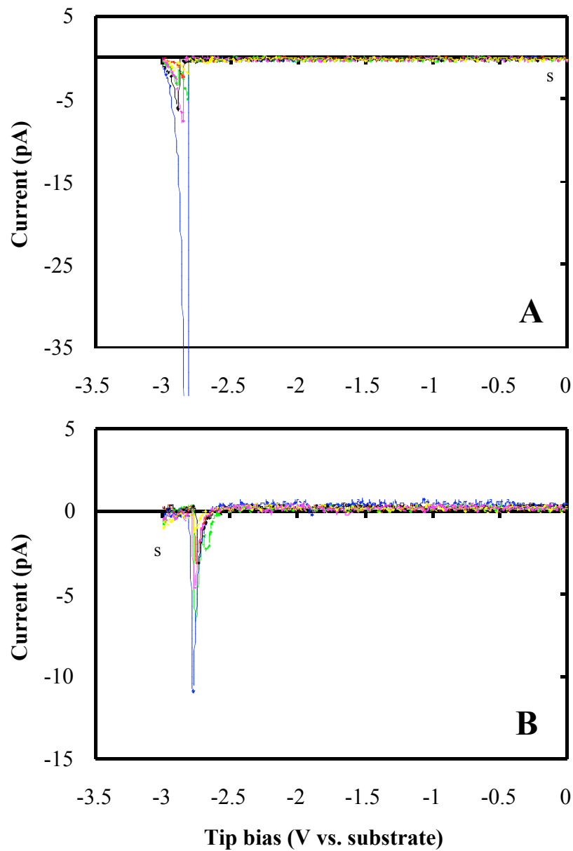
Figure S1. Twelve i-V curves of a SAM of compound I in the negative tip bias region at a Pt tip. A: Six forward scans (black, yellow, blue, red, pink and green); B: Six reverse scans (black, yellow, blue, red, pink and green). The curves represent scans at different locations.
