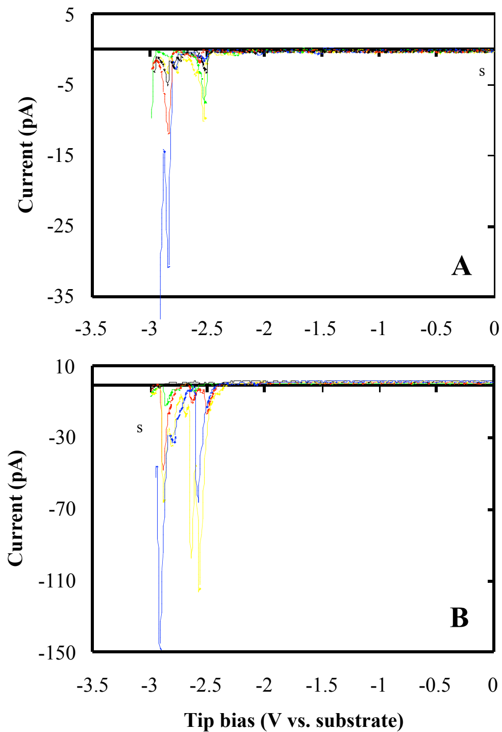
Figure S2. Ten i-V curves of a SAM of compound III in the negative tip bias region at a Pt tip. A: Five forward scans (black, yellow, blue, red and green); B: Five reverse scans (black, yellow, blue, red and green). The curves represent scans at different locations.
