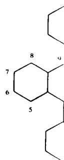
9,10-diphenyl
