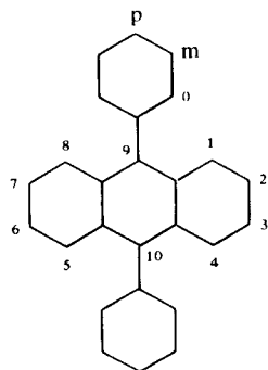
9,10-diphenylanthracene
