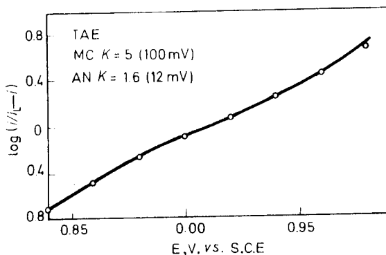
Figure 6. Logarithmic analysis of rotating disc voltammetric wave for oxidation of tetrakis-( p -methoxyphenyl)ethylene at platinum electrode in methylene chloride-0.2 M tetra- n -butylammonium perchlorate
