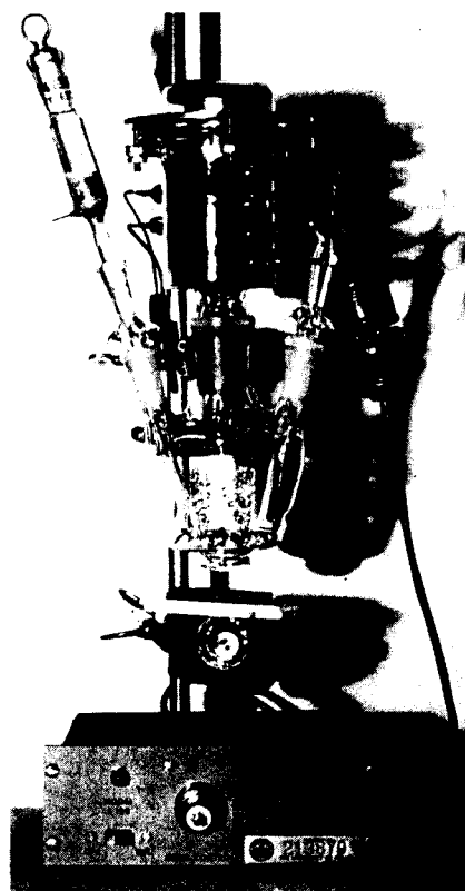
Figure 3. Rotating ring-disk electrode assembly for use in aprotic solvents and closed systems. The entire motor-tachometer assembly is enclosed in the glass envelope. The motor power supply and controller is at the bottom of the picture
