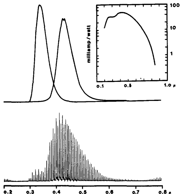
Figure 3. Top: scaled fluorescence spectrum of thianthrene ([TH] = 3.4 \text{ mM} ) and of 2,5-diphenyl-1,3,4-oxadiazole ([PPD] = 1.2 \text{ mM} ) taken in a quartz cuvette using nondegassed acetonitrile as solvent with excitation at 310 \text{ nm} . The true intensity of PPD fluorescence is about 50 times that of TH at these concentrations. Inset: nominal spectral response of the HTV 456 photomultiplier tube which was used to take all spectra shown in figures. Bottom: ecl emission spectrum of the TH-PPD mixed system recorded from 2000 to 8000 \text{ \AA} using a cyclic square wave at 0.2 \text{ Hz} between \pm 3.30 \text{ V} ; [TH] = 7.3 \text{ mM} , [PPD] = 7.0 \text{ mM} .
