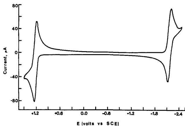
Figure 2. Cyclic voltammogram of the thianthrene-2,5-diphenyl-1,3,4-oxadiazole mixed system. The area of the platinum wire electrode = 0.17 \text{ cm}^2 , [TH] = 1.00 \text{ mM} , [PPD] = 0.94 \text{ mM} , [TBAP] = 0.10 \text{ M} , scan rate = 100 \text{ mV/sec} .
